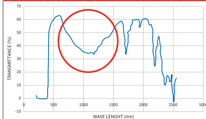
SPECTRA OF SOLARIS PC MW 10mm TWIN WALL CLEAR
