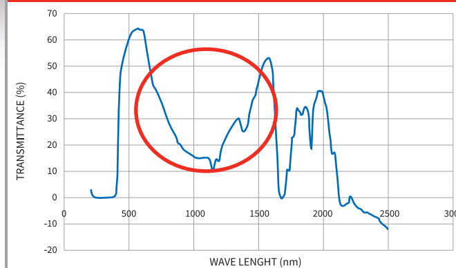
SPECTRA OF SOLARIS SOLID PC 8mm
