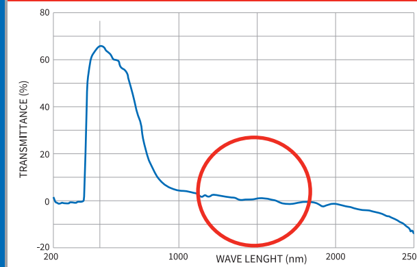
SPECTRA OF SOLARIS PLUS SOLID PC 8mm
