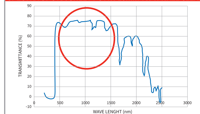
SPECTRA OF STD. SHEET PC MW 10mm TWIN WALL CLEAR
